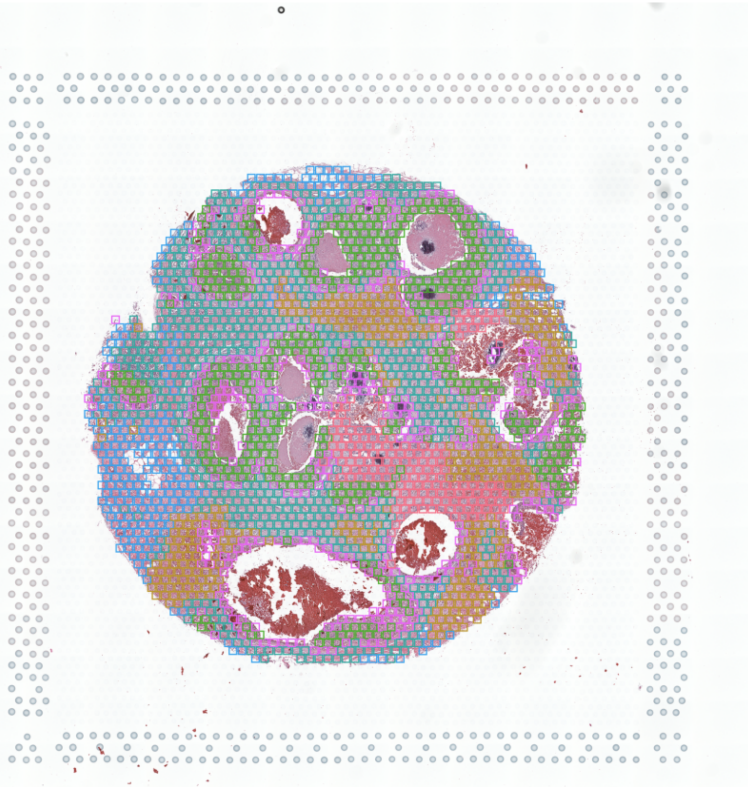
Results from K-Means clustering – 100 \mu m tiles
