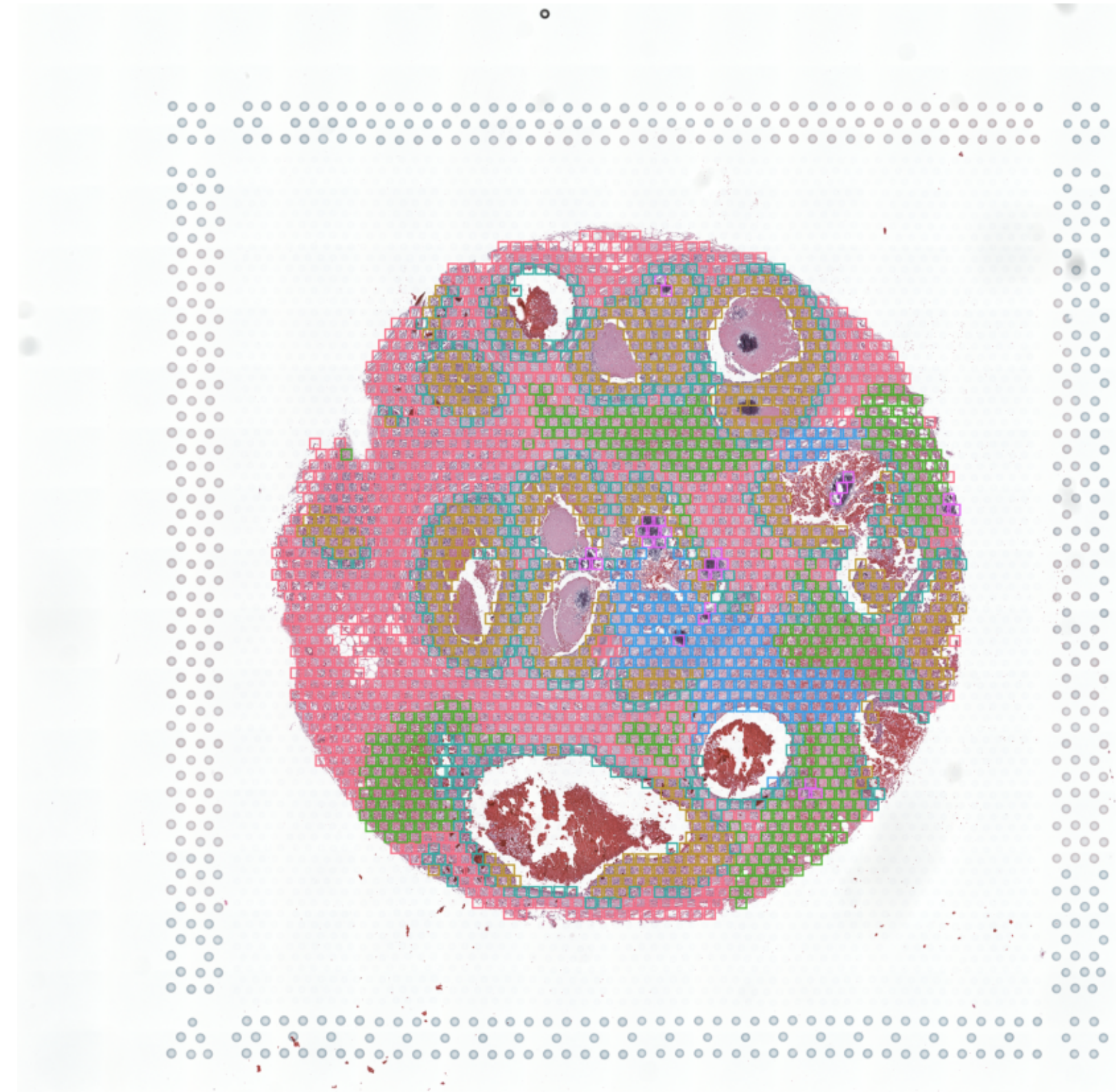
Results from Leiden clustering – 100 \mu m tiles
